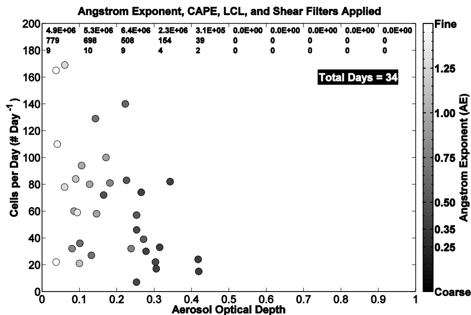
Figure 23. Same as Fig. 15 except that the number of cells for a day is plotted instead of the precipitation flux per cell, only days with AE (440/675 nm) greater than 0.35, CAPE greater than 1000 J Kg -1 , LCL less than or equal to 2.5 Km AGL and wind shear less than 30 m s -1 are included.
