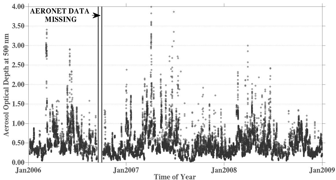
Figure 6. Time series plot of the Aerosol Optical Depth at the IER Cinzana AERONET site. All available 675 nm and 440 nm Level 2.0 data is used to calculate the plotted 500 nm Aerosol Optical Depth. Measurements are conducted every 15 minutes.
