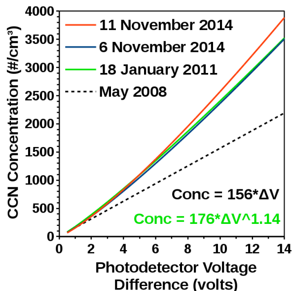
Figure 6: Calibration relationships for the University of Wyoming (UWyo) cloud condensation nuclei (CCN) counter (serial number 107) at 1.0 (theoretical value) supersaturation. The dashed line is the calibration conducted by the UWyo using the supersaturation spectrum method while the solid lines are the calibrations conducted by the University of North Dakota (UND) at a single supersaturation. The legend provides the calibration date. The equations (lower right) provide the relationship between photo-detector voltage difference ( \Delta V ) and the CCN concentration (Conc) for the May 2008 (black) and January 2011 (green) calibrations. Plot created using LibreOffice software.
