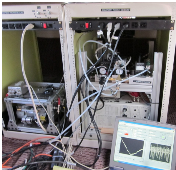
Figure 11: Image of the sulfur hexafluoride (SF 6 ) analyzer in the back racks on the Citation Research aircraft conducting ground tests during the summer of 2010. The pump and constant pressure inlet system are on the left side of the image. The Electron Capture Detector (ECD) and hydrogen bottle are on the right side of the image.
