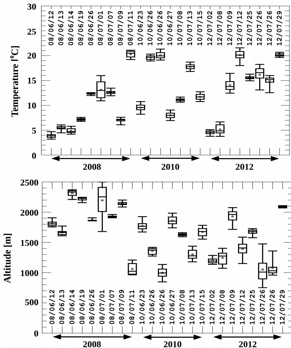
Figure 9: Statistical distributions of just below cloud base ambient air temperature (Top) and altitude (bottom) of developing cumulus clouds in North Dakota. Box-and-whiskers and date text are similar to Figure 8. Cloud base altitude given above mean sea level (MSL). Plot created using the Airborne Data Processing and Analysis software package (ADPAA).
