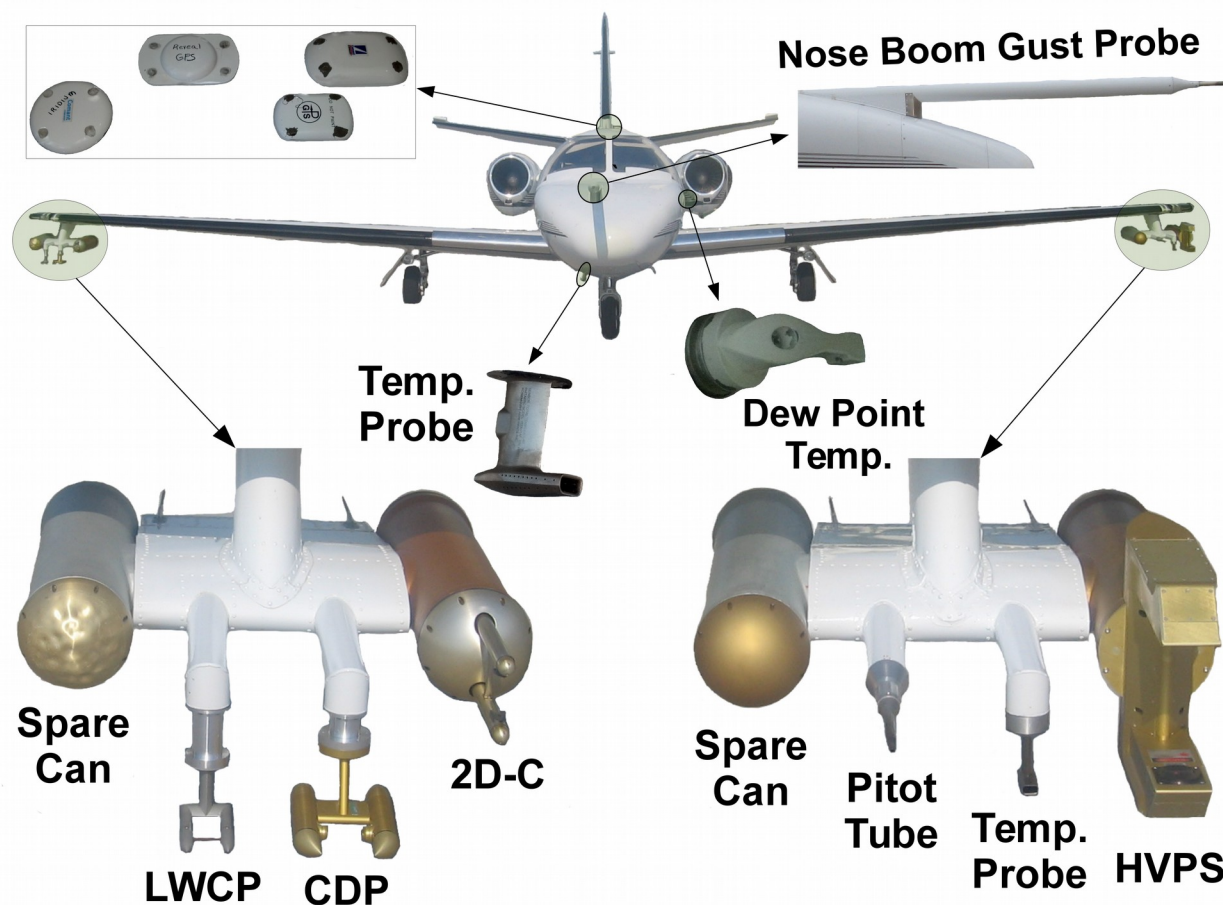
Figure 5: Diagram of the Citation Research Aircraft configuration for 2010, the only year of project participation. An analog-to-digital board (A/D) records voltage outputs from the Dew Point Temp instrument and Temp. Probe. Acronyms are defined in the bullet list of instruments. Image is created using LibreOffice and GNU Image Manipulation Program (GIMP) software.
