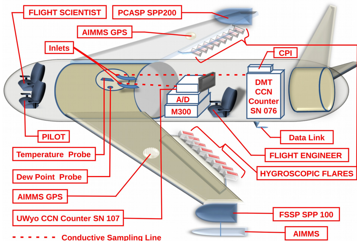
Figure 4: Diagram of the Cessna 340 aircraft configuration for 2012. The 2010 and 2008 aircraft configuration is similar except the Droplet Measurement Technologies (DMT) cloud condensation nuclei (CCN) counter and aircraft integrated meteorological measurements system (AIMMS) probe are not on the aircraft. A DMT constant pressure inlet (CPI) system maintains the DMT CCN counter at a constant pressure of 700 hPa. Flexible conductive tubing of 6.35 mm (0.25 inch) diameter connects the reverse facing inlets to the CCN counters and two additional ports (not shown) on the window insert provide the exit for the air sample. An analog-to-digital board (A/D) records voltage outputs from the University of Wyoming (UWyo) CCN counter, the Dew Point Probe, and Temperature Probe. The Data Link system uses a 465 MHz antenna to down link data. The bullet list of instruments defines all acronyms. Image created using LibreOffice software.
