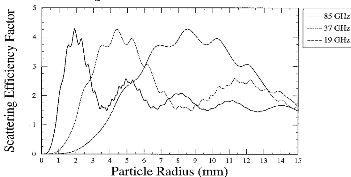
Figure 7. Scattering efficiency factor for spherical ice and ash particles as a function of radius. The index of refraction of ice [Tiuri et al. , 1984] is different than the index of refraction of volcanic ash [Adams et al. , 1995], which results in different scattering efficiency factors for ice and ash particles.
