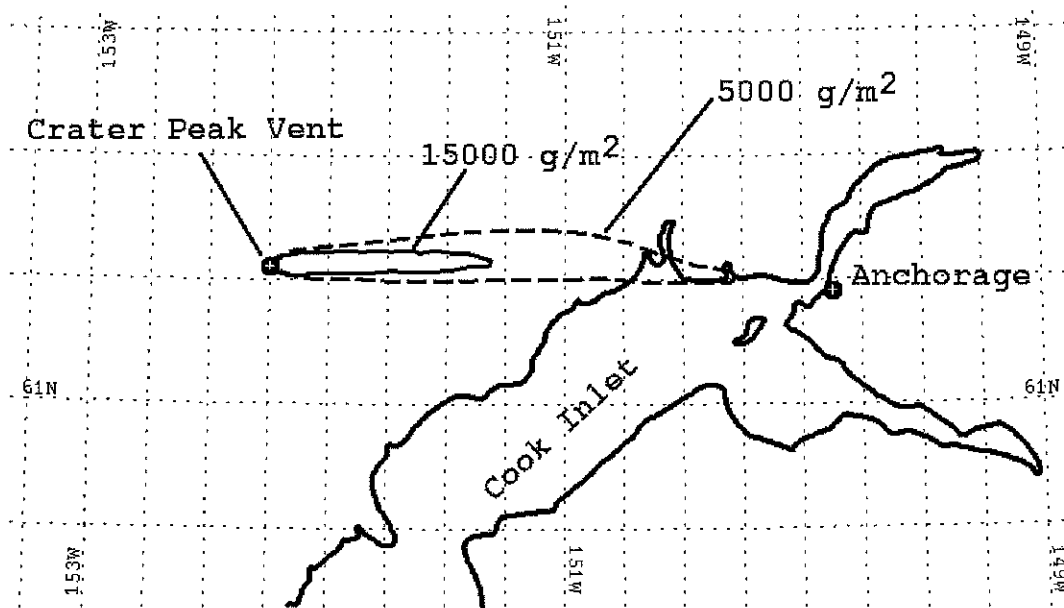
Figure 8. Isomass maps ( \text{g}/\text{m}^2 ) of the August 19, 1992 Crater Peak/Spurr volcanic cloud as estimated from SSM/I data using the modified rain fall rate equation (top) and ground sampling of the ashfall blanket (bottom) [R. G. McGimsey, personal communication]. The pixels in the SSM/I image are about 12.5 by 12.5 kilometers. The difference observed between the SSM/I data and the ground sampling data may be due to a wind shear. Note that the value of the 15000 contour line is only my estimate.
