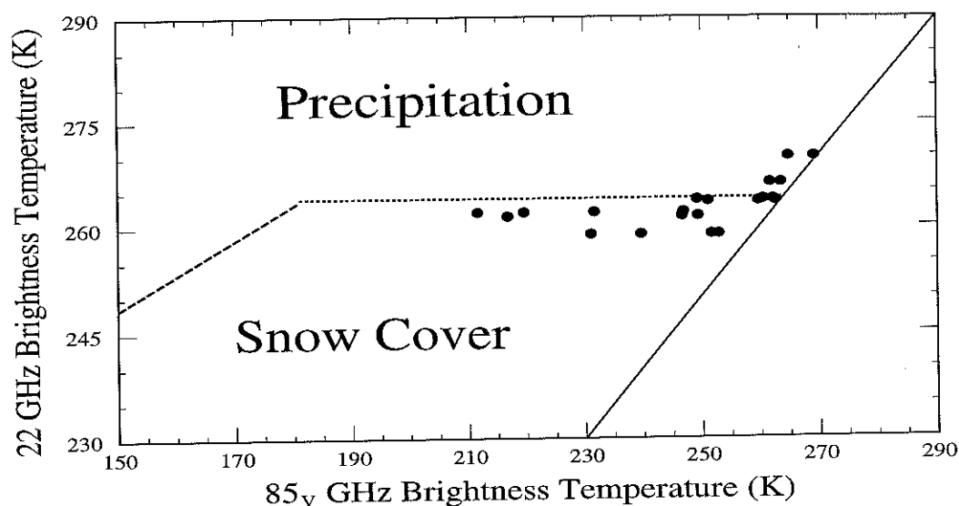
Figure 5. The solid circles are pixels values from the August 19, 1992 Crater Peak/Spurr volcanic cloud. The solid line denotes the separation between scatterers (left) and absorbers (right). The dashed lines are based on empirical equations that are generally used to separate precipitation and snow cover [Ferraro et al. , 1994b].
