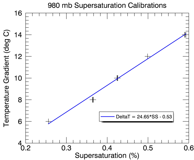
Figure 9: Supersaturation calibrations done between October 28 th and November 5 th , 2016 in the University of North Dakota Instrumentation Laboratory (ambient pressure of approximately 980 hPa ). Three data points are taken at each \Delta T . A least squares linear fit is used to determine the given supersaturation calibration equation.
