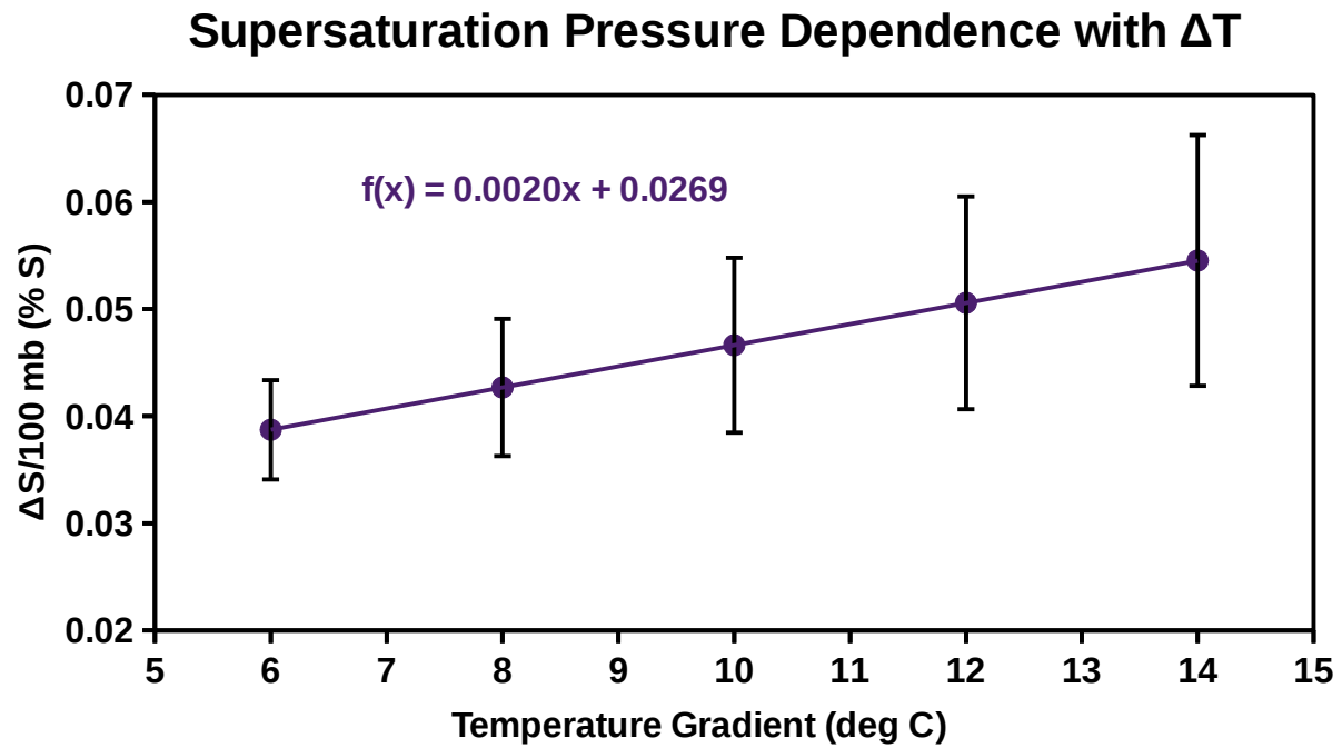
Figure 13: Calculated supersaturation pressure dependencies are shown at their corresponding \Delta T conditions. \Delta S represents the change in supersaturation percentage. A linear fit is applied to the data to show the relation of the pressure dependence to \Delta T .
