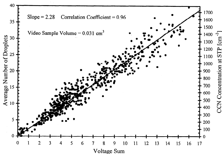
Figure 2. Plot of the photodetector voltage sum versus the number of cloud condensation nuclei within the video sample volume. Data from six independent calibration runs, of 100 air samples each, are shown. NaCl aerosol is used during calibration.
