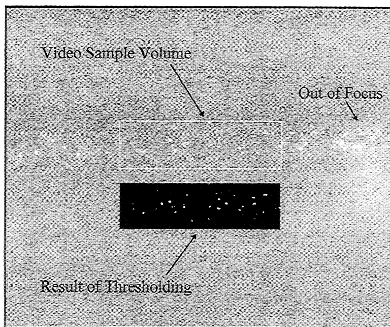
Figure 1. A typical video image of droplets in the static thermal-gradient diffusion chamber. The top part of the image is the raw gray scale digital image. The white rectangle outlines the area in which droplets are counted. Below, the gray scale image is the corresponding black and white image produced by applying the brightness threshold value.
